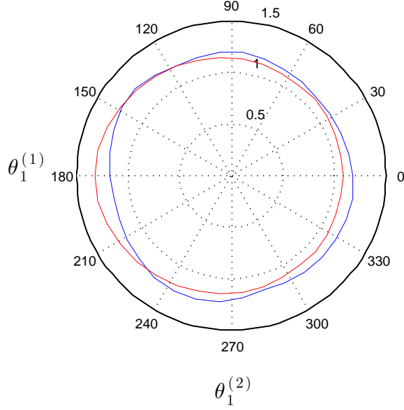
Figure 1: f_{\theta_1^{(1)}, \theta_1^{(2)}} and \hat{f}_{\theta_1^{(1)}, \theta_1^{(2)}} under Specification 1.
