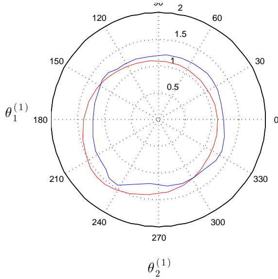
Figure 2: f_{\theta_1^{(1)}, \theta_2^{(1)}} and \hat{f}_{\theta_1^{(1)}, \theta_2^{(1)}} under Specification 1
