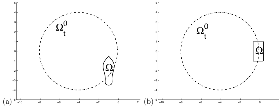
FIG. 1. Scatterer \Omega and test domain \Omega_t^0 used in reconstruction simulations. The obstacle \Omega in (a) is used for Dirichlet, Neumann, and impedance obstacle reconstructions. The scatterer shown in (b) is used for inhomogeneous media reconstructions.
