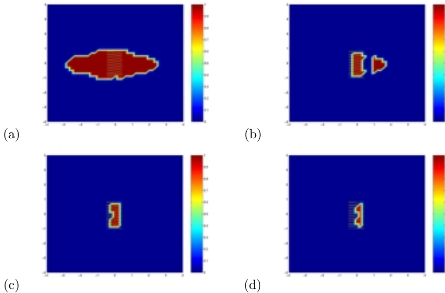
FIG. 9. (a)–(d) We show several thresholded versions of the function F for the reconstruction of an inhomogeneous medium, where we used the thresholds C = 0.1 , C = 0.06 , C = 0.05 , and C = 0.045 .
