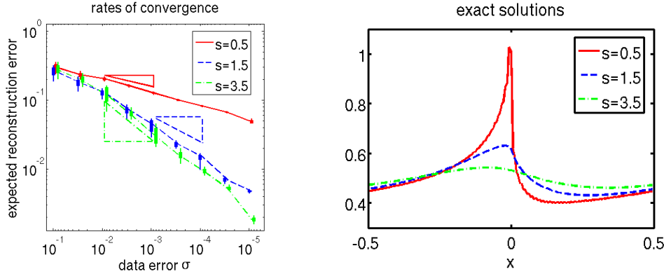
FIG. 5.1. left panel: rates of convergence of (\mathbf{E} [\|a^\dagger - \hat{a}_{k_{\text{bal}}}\|^2])^{1/2} as \sigma \rightarrow 0 for different smoothness of exact solution. The triangles indicate the rates predicted by theory and the bars the empirical standard deviations of the reconstruction error. right panel: exact solutions.
