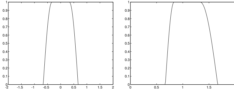
Figure 17: Plot of the windows V(\omega) (left) and W(r) (right).
