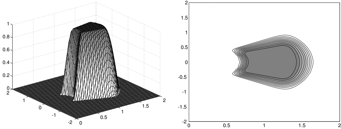
Figure 4: Basic curvelet \hat{\psi} in frequency domain (left) and its support (right).
