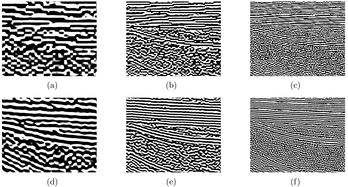
Figure 12: Comparisons of subband reconstruction in the first three levels from coarse scale to fine scale by wavelet transform (upper row) and curvelet transform (lower row).
