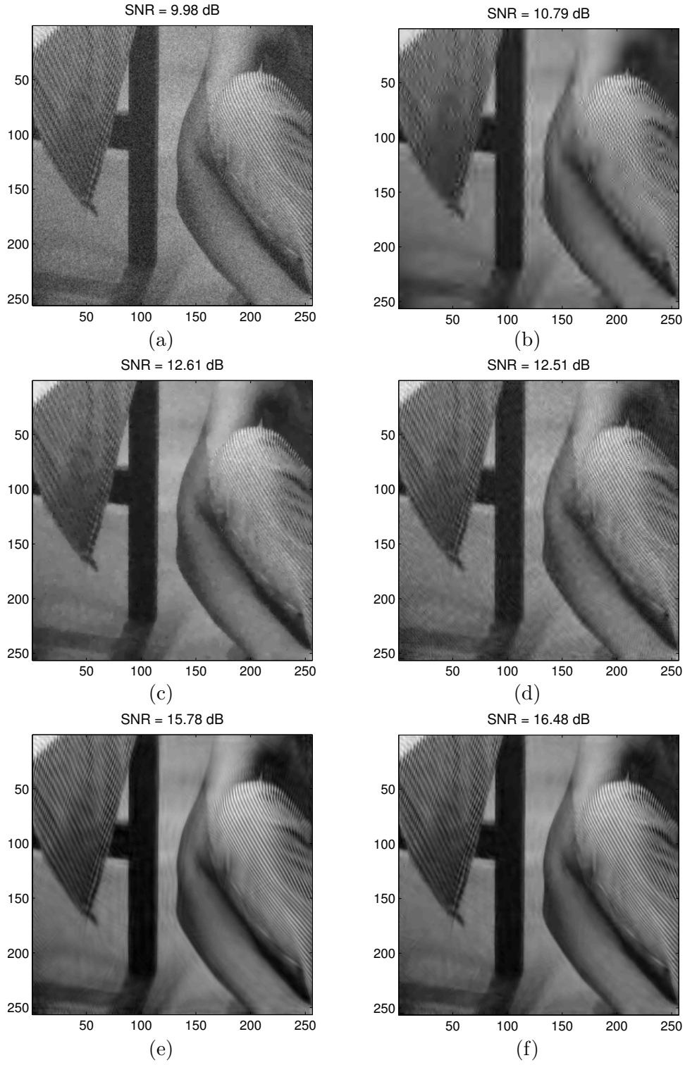
Figure 10: Image denoising. (a) Noisy image, (b) wavelet denoising, (c) TV-diffusion denoising, (d) contourlet denoising, (e) curvelet denoising, (f) TV-combined curvelet denoising.
