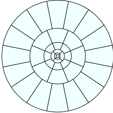
Figure 3: Tiling of the frequency domain into wedges for curvelet construction.
