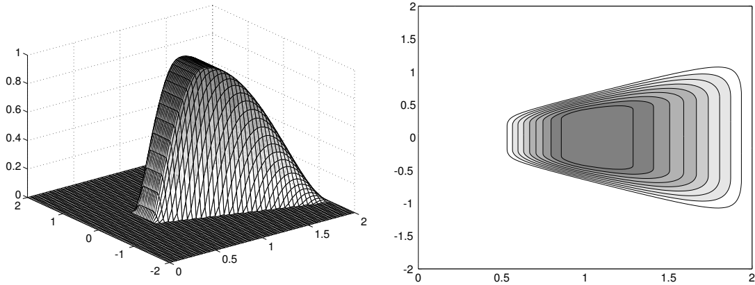
Figure 8: Basic curvelet \widehat{\phi}_{0,0,0} (left) and its support (right) adapted to the Cartesian arrays in frequency domain.
