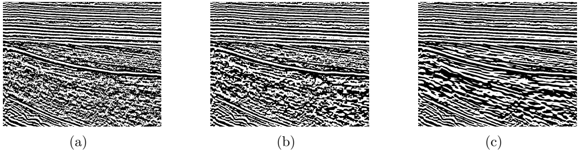
Figure 11: Comparison of seismic denoising. (a) Original data, (b) wavelet denoising, (c) curvelet denoising.
