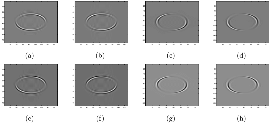
Figure 14: Curvelet coefficients of an instant wave field at the coarsest curvelet detail scale. (a)-(h) denotes eight different directional subbands in this curvelet scale.
