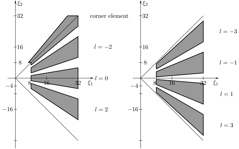
Figure 9: Supports of the functions \hat{\phi}_{4,\mathbf{k},l} for l = -3, \dots, 3 , and one corner element.
