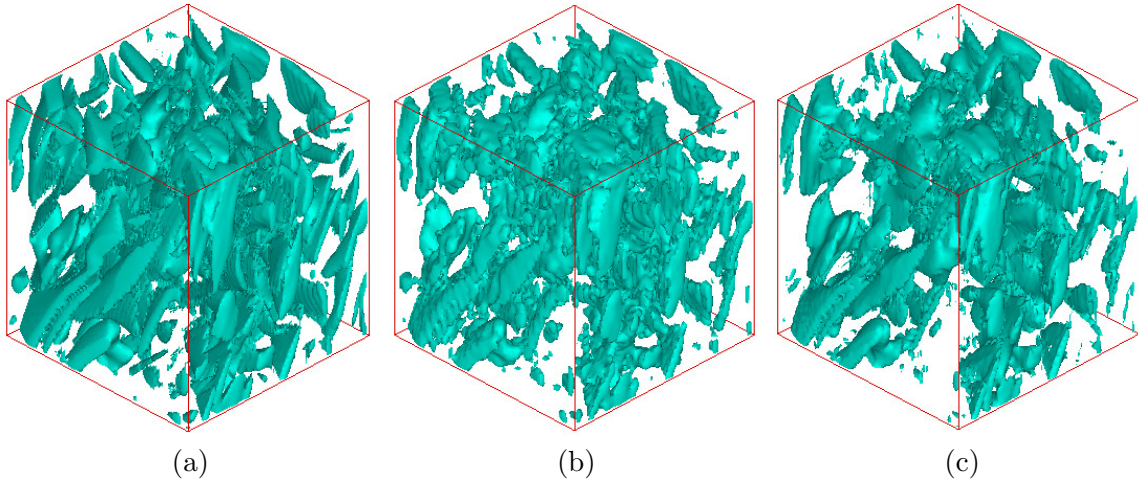
Figure 13: Extraction of coherent fields from turbulent flows. (a) Original flow, (b) coherent components by wavelets, and curvelets.
