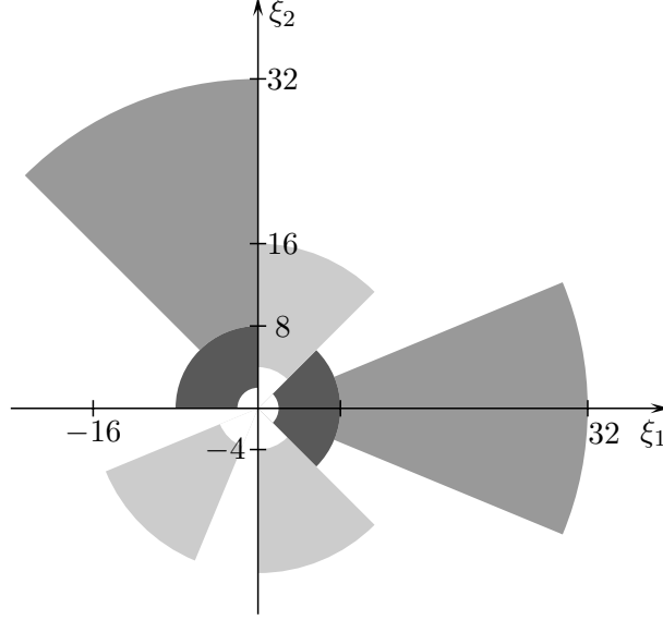
Figure 6: Maximal supports of \widehat{\phi}_{2,\mathbf{k},0} and \widehat{\phi}_{2,\mathbf{k},5} (dark grey); of \widehat{\phi}_{3,\mathbf{k},3} , \widehat{\phi}_{3,\mathbf{k},6} and \widehat{\phi}_{3,\mathbf{k},13} (light grey); and of \widehat{\phi}_{4,\mathbf{k},0} and \widehat{\phi}_{4,\mathbf{k},11} (grey). The translation index \mathbf{k} \in \mathbb{Z}^2 does not influence the support of the curvelet elements.
