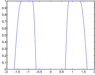
Figure 2: Plot of a Meyer wavelet \hat{\psi}(\xi) in frequency domain.
