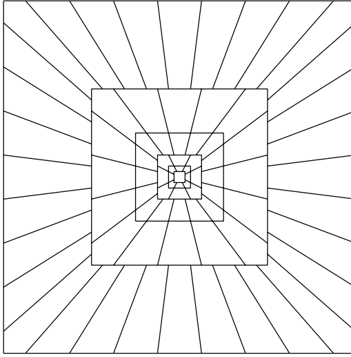
Figure 7: Discrete curvelet tiling with parabolic pseudo-polar support in the frequency plane.
