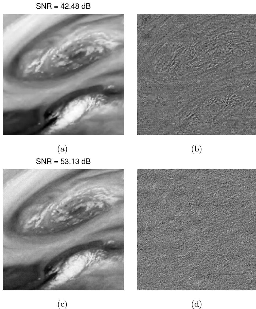
Figure 16: Compressed sensing in remote sensing. (a) Recovery by iterative wavelet thresholding, (b) recovery error by the wavelet method, (c) recovery by iterative curvelet thresholding, (d) recovery error by the curvelet method.
